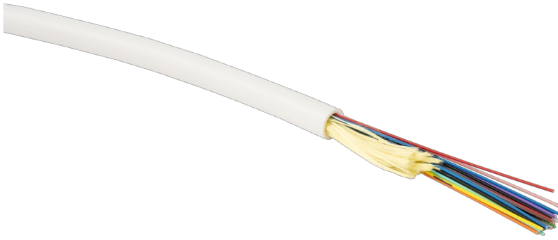
Indoor Tight Buffered Cable Internal, CPR, Bca, Pre-terminated, Bend-insensitive Rugged Drop Cable G.657a1 Hexatronic
