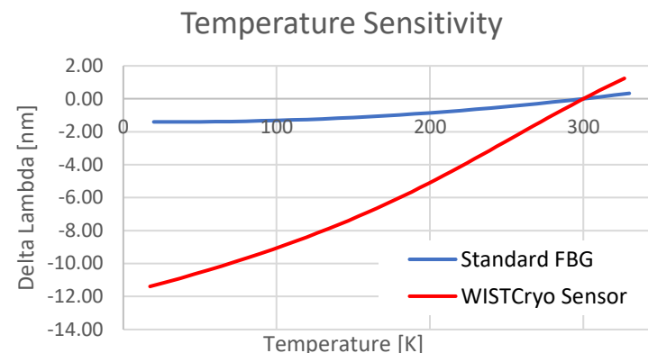
Showing superior WISTCryo sensitivity vs. a standard FBG sensor
